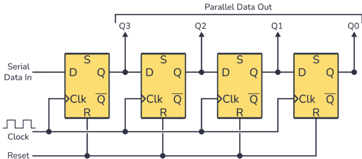
[6] Figure 2 Serial in parallel out shift register
